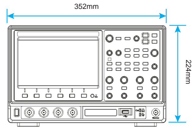
Figure 1 Front View
