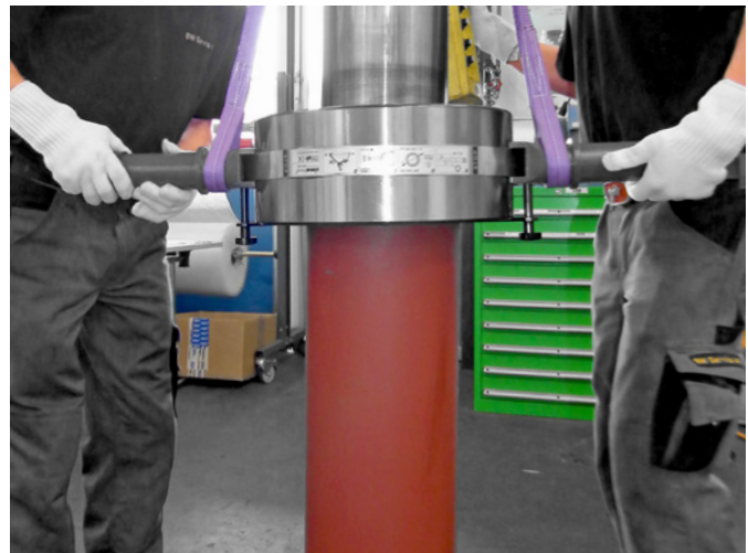
The Bearing Handling Tool BHT allows the heavy, pre-heated roller bearing to be safely lifted and accurately positioned on a turbine shaft.
