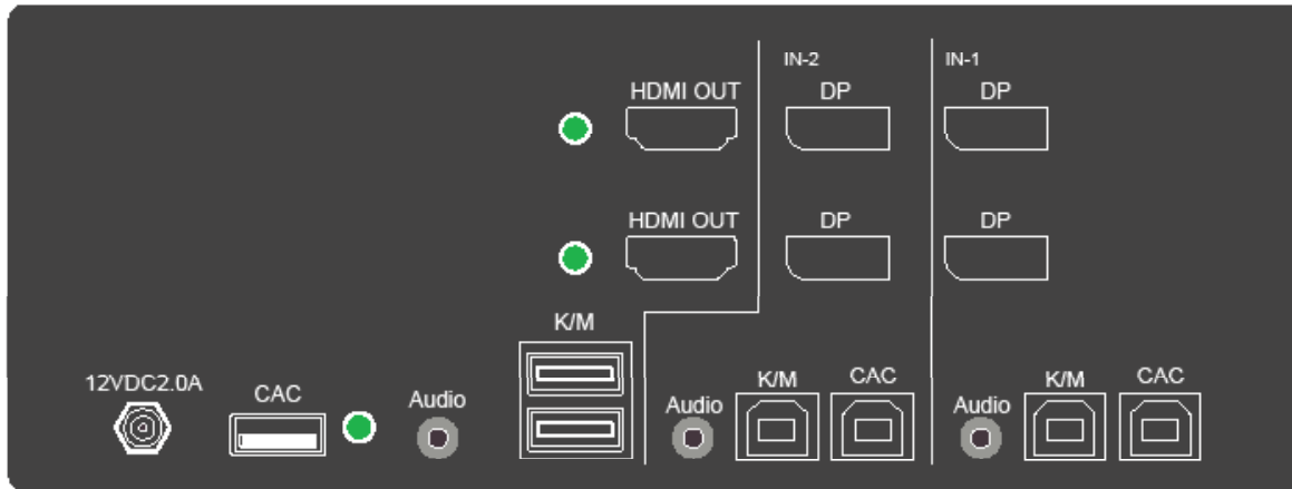
SDHN-2D-P Back
