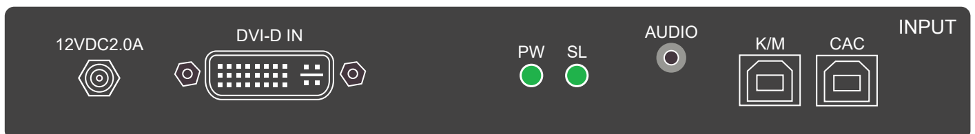
Figure 4-2: SDVN-1S-P Rear panel
