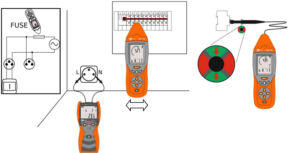
Fig. 27 Identifying safety devices in a switchboard.
