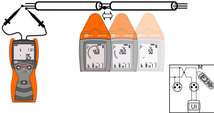
Fig. 26 Locating shorted cores in a conductor.
