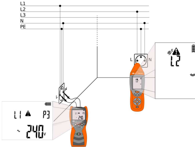
Fig. 31 Phase identification.
