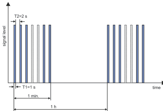
Fig. 52. An example of low-frequency signal transmission.
