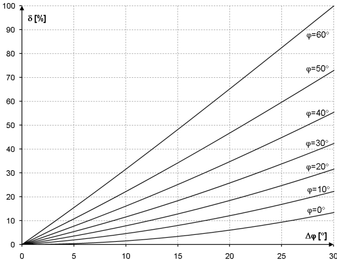
Fig. 64. Additional uncertainty due to the phase error, depending on the phase angle.
