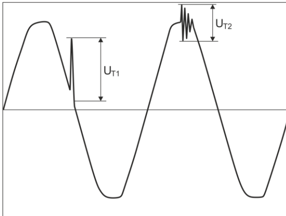
Fig. 45. Method of determining the amplitudes of transients.
