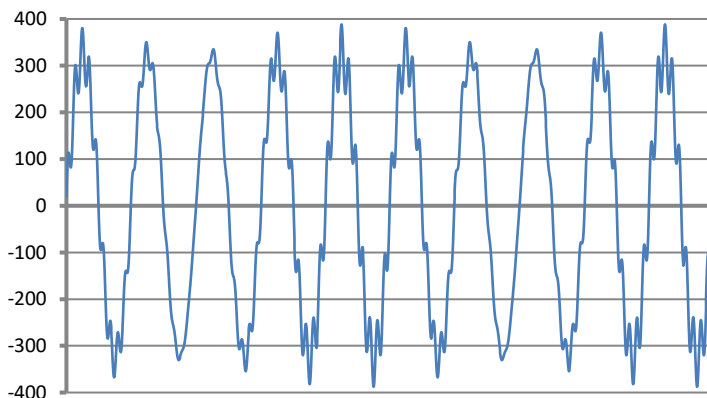
Fig. 51. The effect of 9th harmonic interaction (450 Hz, 10% Unom) and interharmonic 460 Hz (10% Unom). The apparent change in the voltage envelope with frequency of 10Hz that may cause flicker (Unom = 230 V RMS, 50 Hz).
