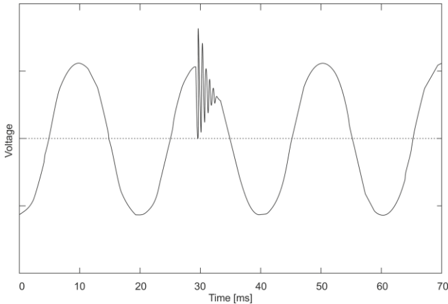
Fig. 59. An example of a transient after switching capacitor banks.
