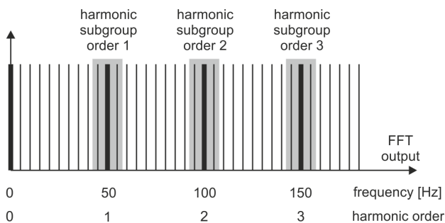
Fig. 43. Determining harmonics subgroups (50 Hz system)
