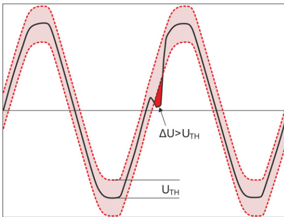
Fig. 46. Detecting waveshape variation events.
