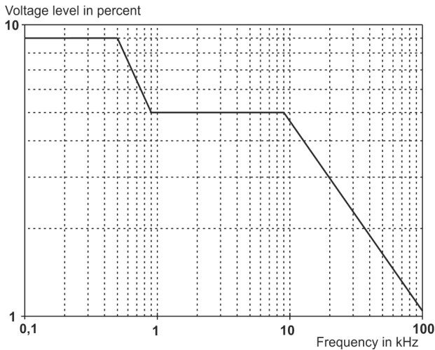
Fig. 53. Allowable levels of mains signalling according to EN 50160 standard.
