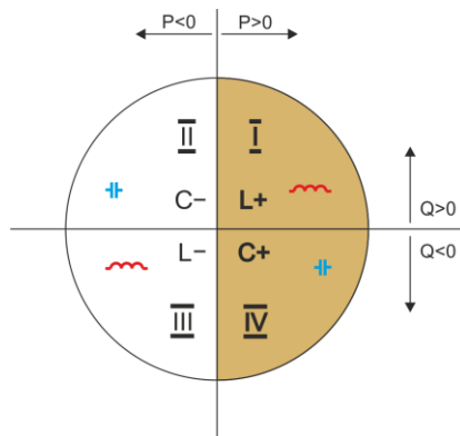
Fig. 50. Four-quadrant division of power and energy flow.
