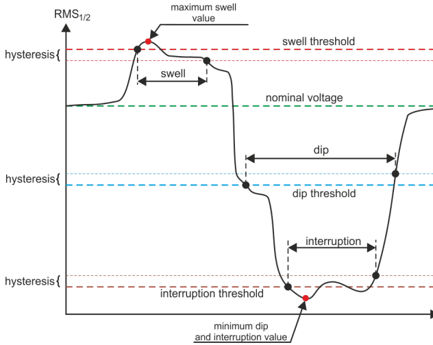
Fig. 55. Voltage swells, dips and interruptions
