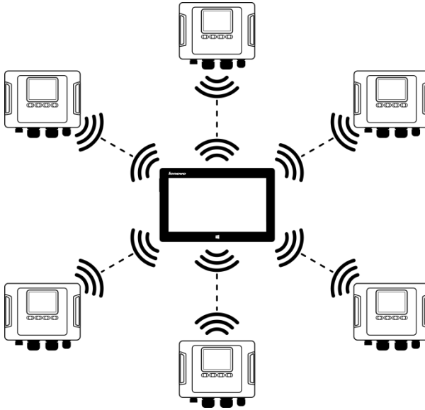
Fig. 33. Direct connection: tablet (AP) ⇔ multiple analyzers (clients).
