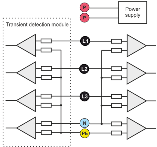
Fig. 42. Voltage inputs (with transient module) and AC adapter
