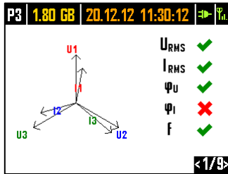
Fig. 5. Screen 1 with a phasor diagram and indicators of connection correctness.
