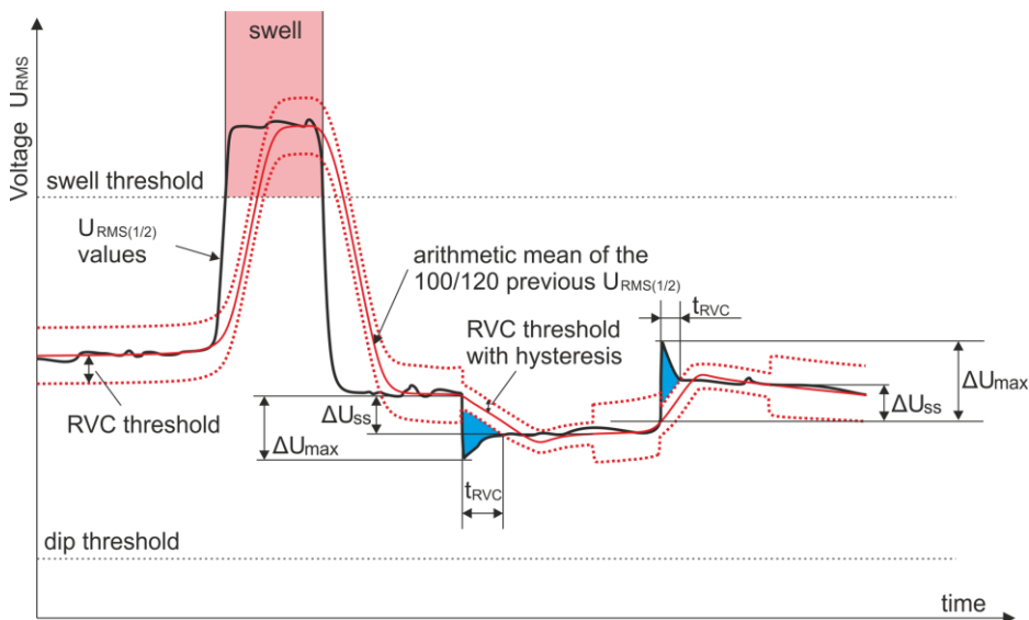
Fig. 57. Rapid Voltage Changes (RVC) - example.
