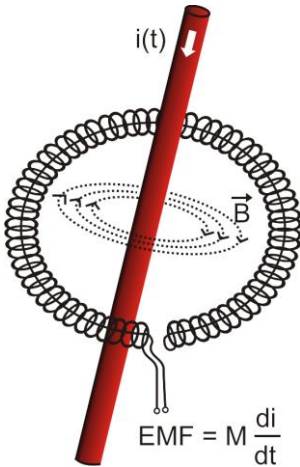
Fig. 49. Rogowski coil
