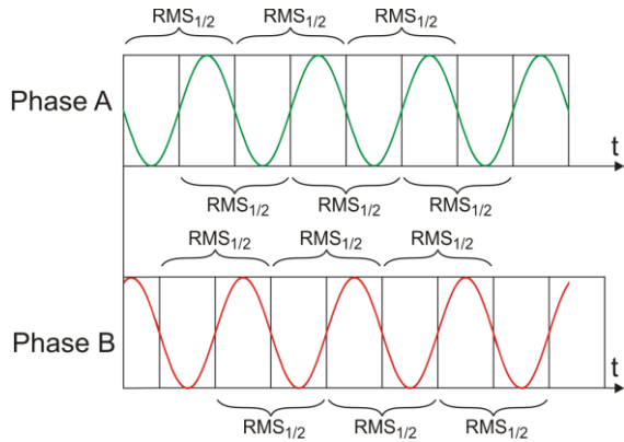
Fig. 56. Determining values of U_{RMS(1/2)}
