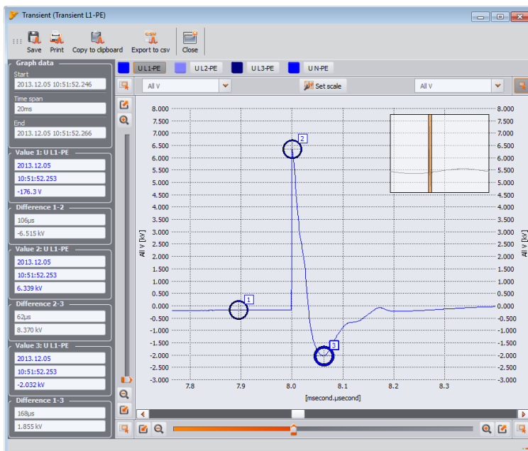
Fig. 58. Example of lightning surge.
