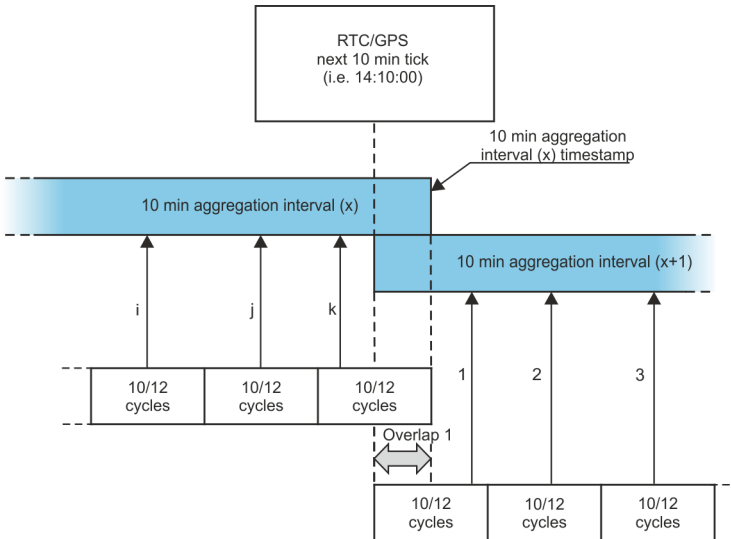
Fig. 61. Determining the averaging intervals longer than 10 seconds (with the 10-minute averaging).
