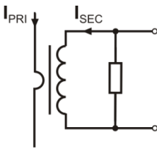
Fig. 48. CT probes with voltage output
