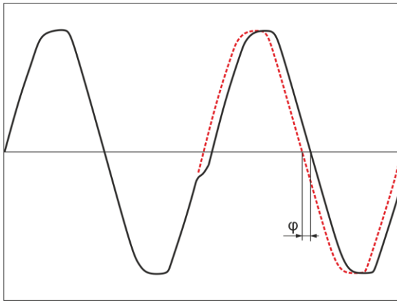
Fig. 47. Phase jump.
