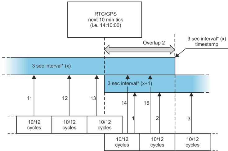
Fig. 62. Determining the averaging intervals shorter than 10 seconds (with the 3-second averaging).
