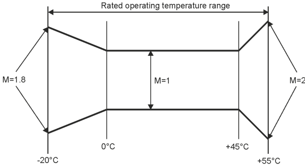
Fig. 63. Basic uncertainty multiplier M as a function of ambient temperature.
