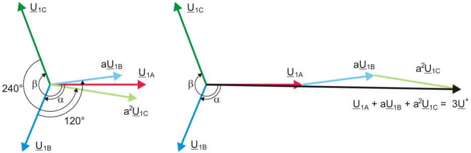
Fig. 54. Example of determining positive sequence component.
