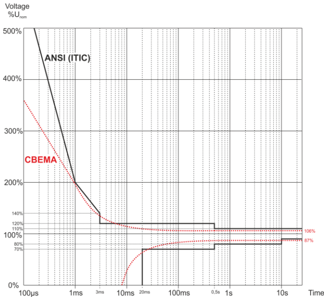
Fig. 60. Voltage tolerance curves: ANSI (ITIC) and CBEMA.
