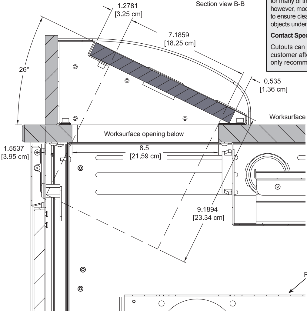
Overbridge Section view B-B
