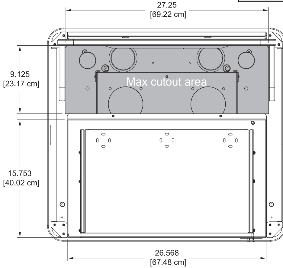
Top View Surround worksurface Max cutout area
