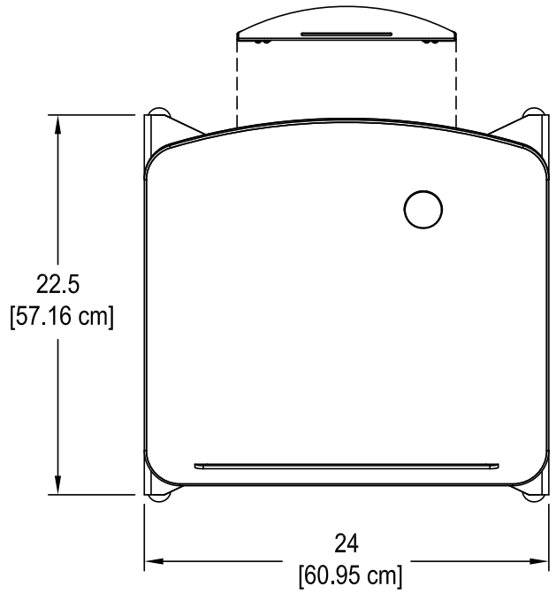
Removable audience-side panel
