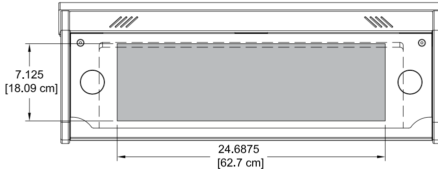
Overbridge panel cutout area
