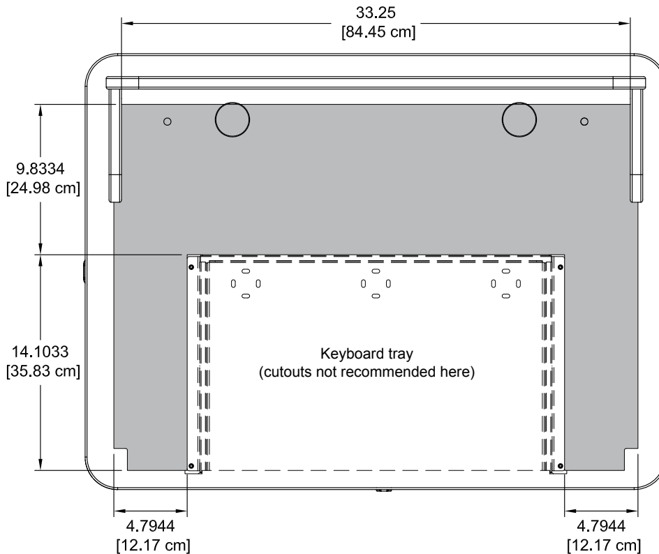
Worksurface cutout area
