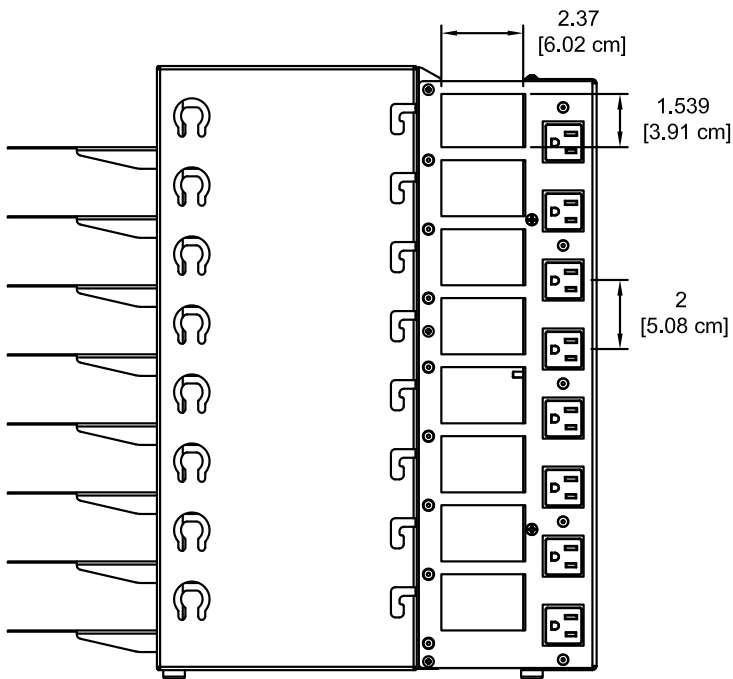
8 power outlets
