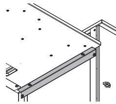
Stepped-Height Bracket (connects 29"H console to 36" console) 68205
