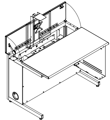
42" single desk with ADA clearance
