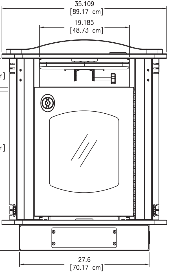
42" LINK Lectern with Toe Kick
