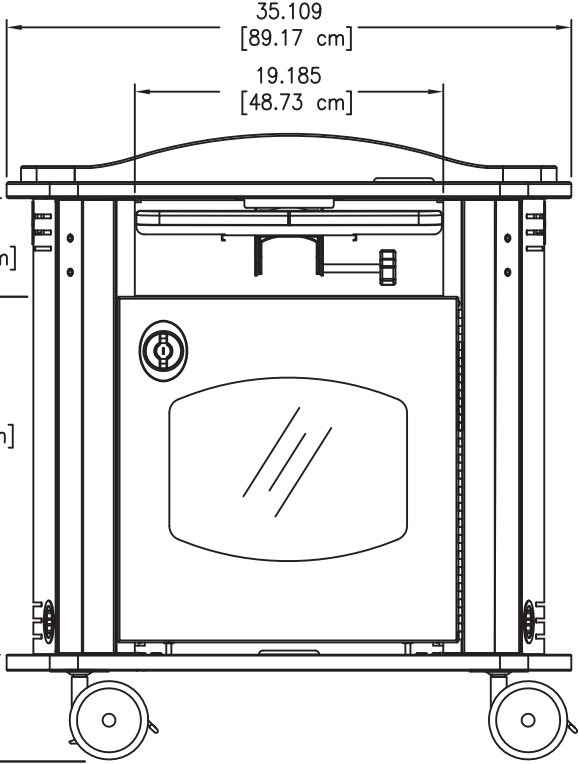
42" LINK Lectern with Toe Kick
