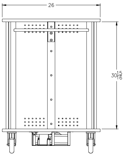
Left-side view
