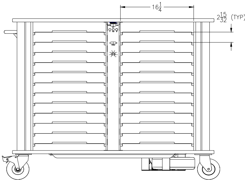
(shown without doors)
