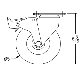
5" Balloon Wheel
