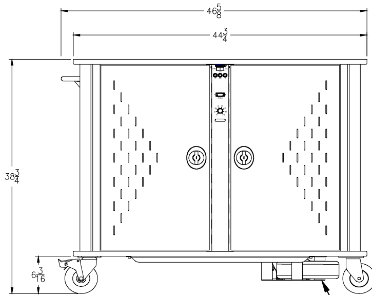
Instructor-side view
