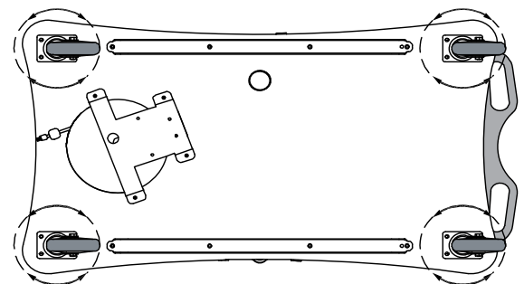
(BW) = 4 swivel wheels (provides more maneuverability in tight spaces, but less control when mobile)
