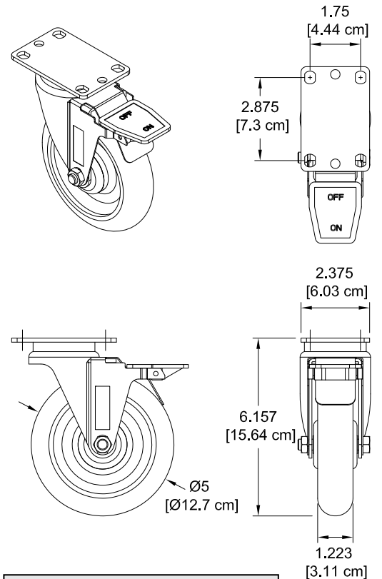
5" Balloon Wheel
