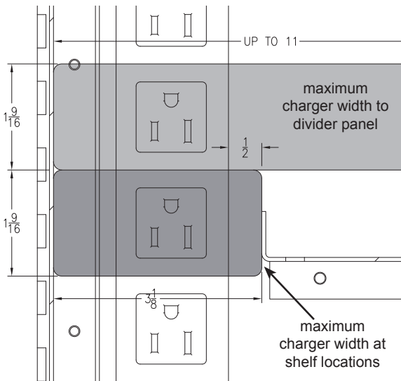
outlet spacing on each 16-outlet power unit
