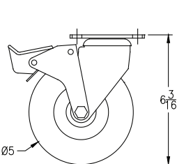
5" balloon wheels
