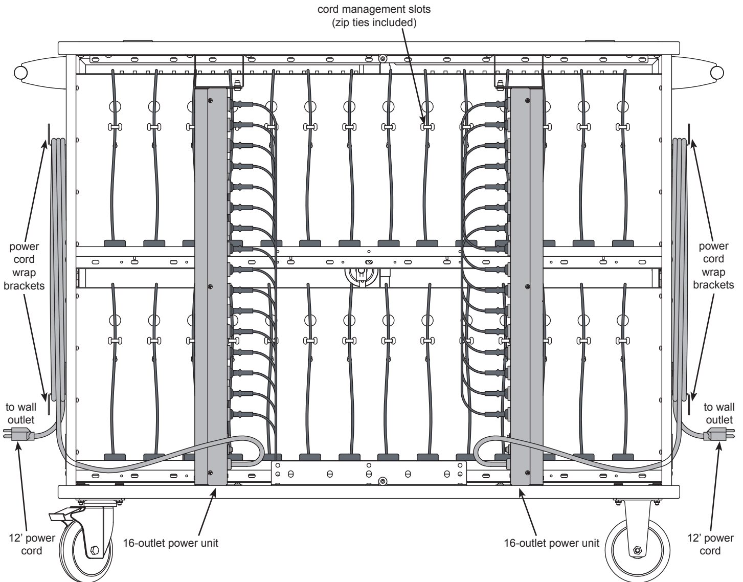
power-side view (shown with doors removed)
