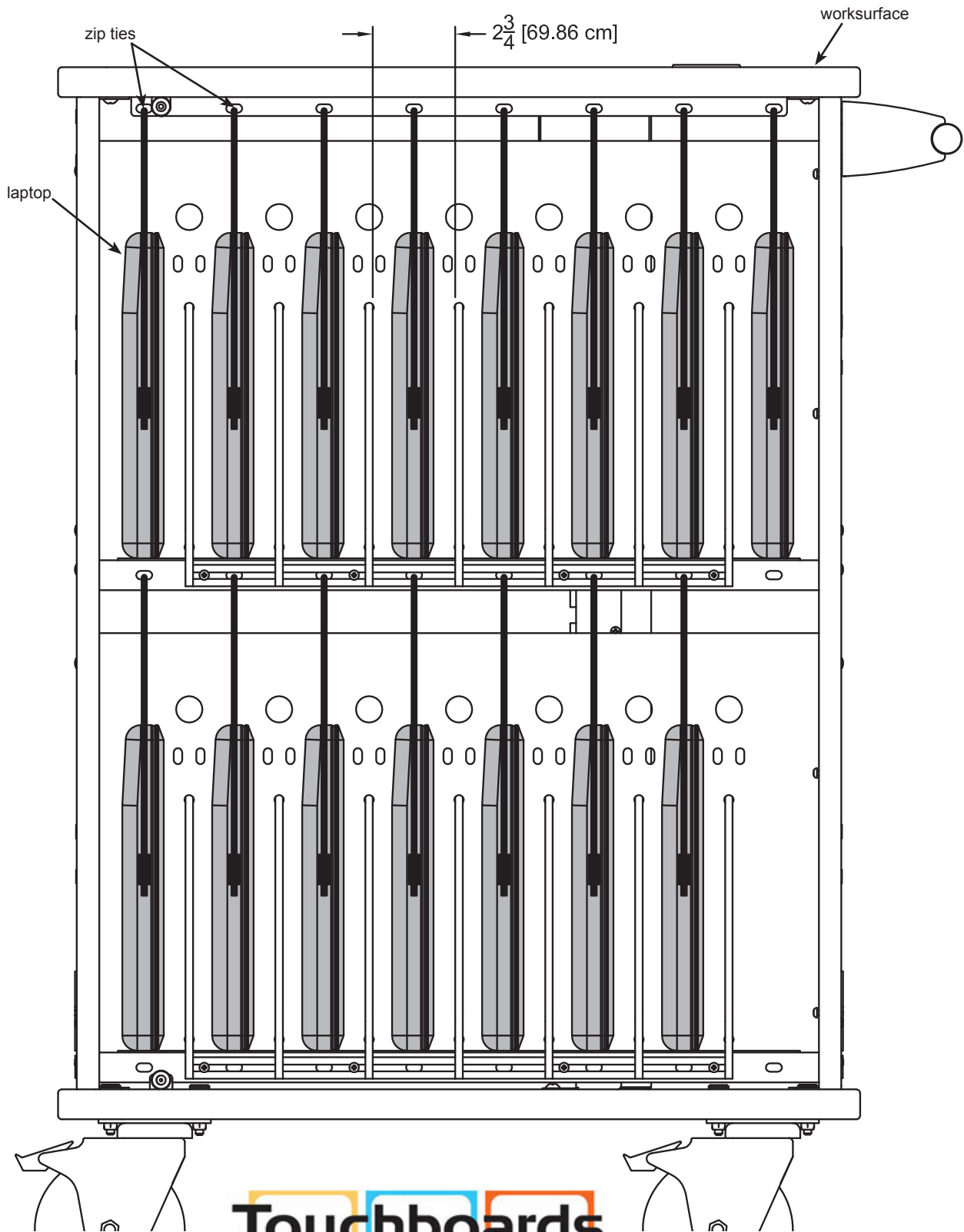
vLT-15 cord management student-side view (shown without door for clarity)
