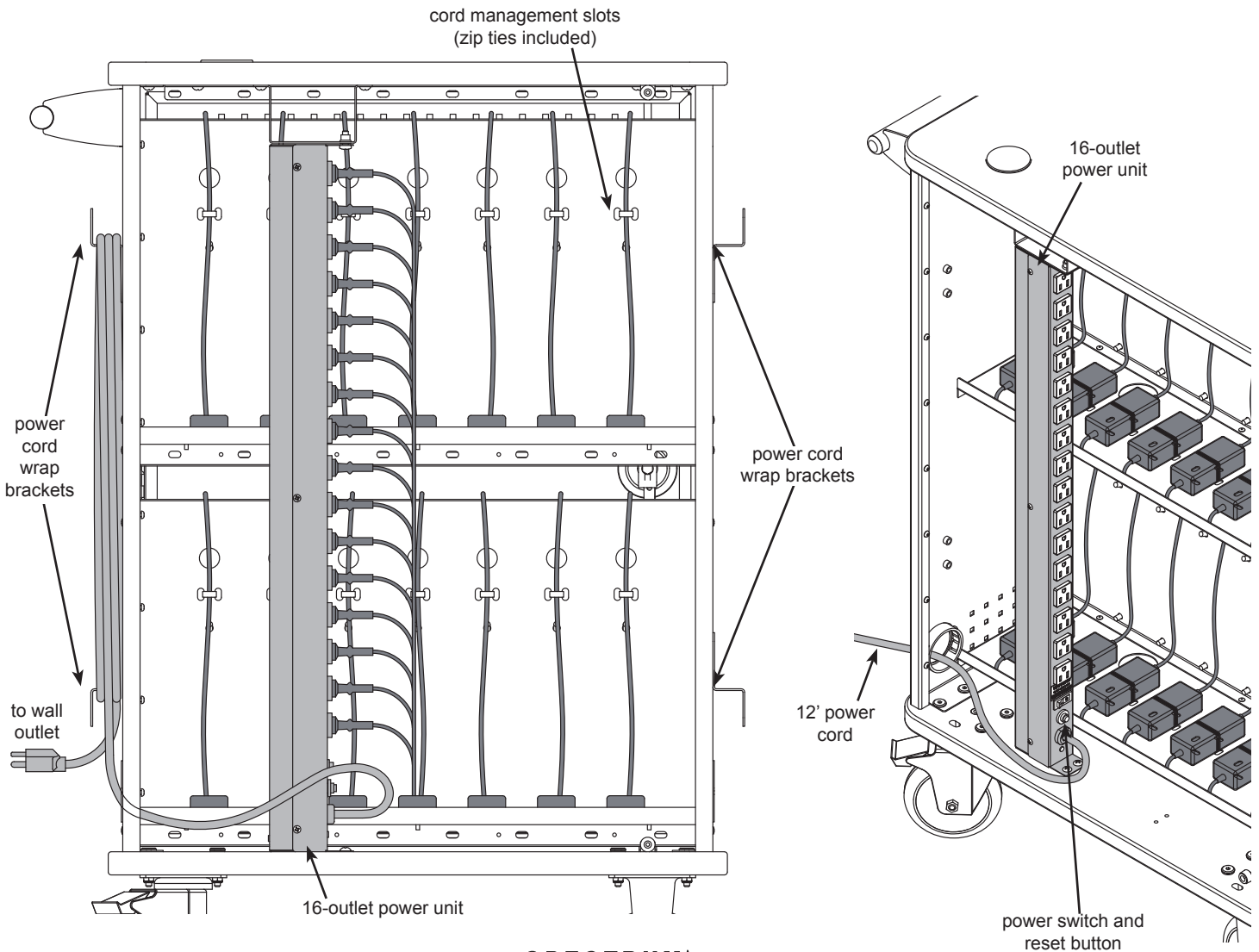
power-side views (shown with door removed)
