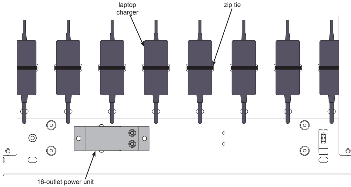
top view of cord management tray
