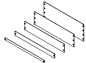
Rack-Mount Blanks (fills rack spaces where components are not needed) 97516 - (½ RU) 97510 - (1RU) 97511 - (2RU) 97512 - (3RU) 97513 - (4RU)
