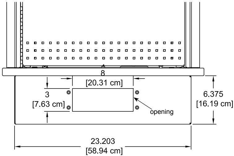
Toe Kick front view
