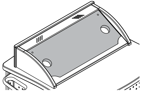
Overbridge Insert Panel for overbridge version only-contact Spectrum to specify cutout size(s) and position(s)-overbridge not available separately (includes two 2" grommets with covers) 96501 - blank panel 96501mod - panel with cutout(s)
