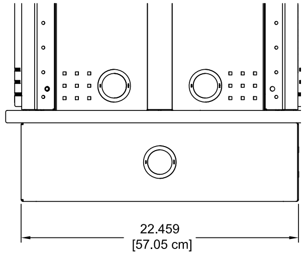
Toe Kick side view
