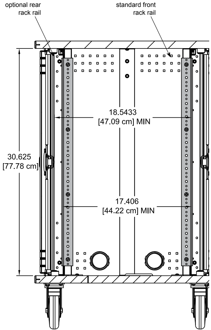
CPL section view
