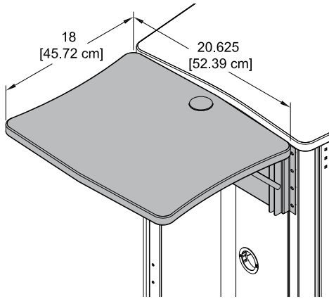
Flip-up Shelf adjustable-height, mounts on left or right 18"W x 20.625"D (50 lbs max load) 55219
