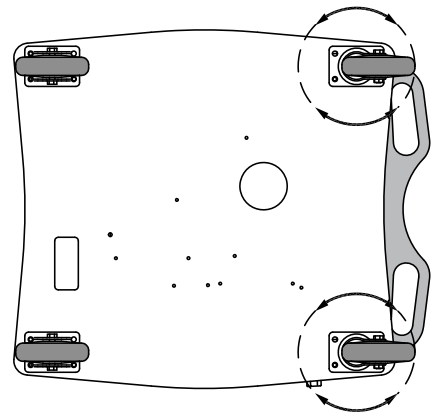
SR 5" Balloon Wheels (2 rigid, 2 swivel) Provides more control when mobile, but less maneuverability in tight spaces
