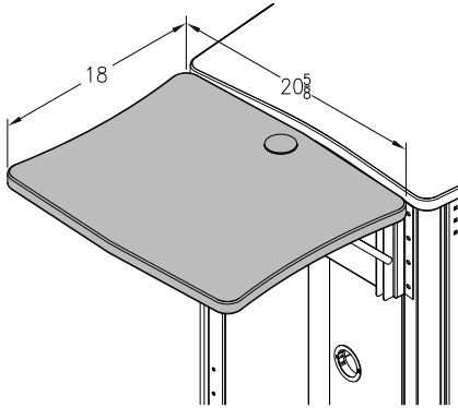
Flip-up Shelf adjustable-height, mounts on left or right 18"W x 20.625"D (50 lbs max capacity) 55219
