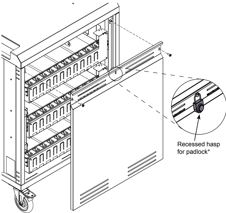
Power-side locking access panel
