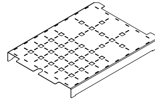
(2) 0147925 Universal panel
