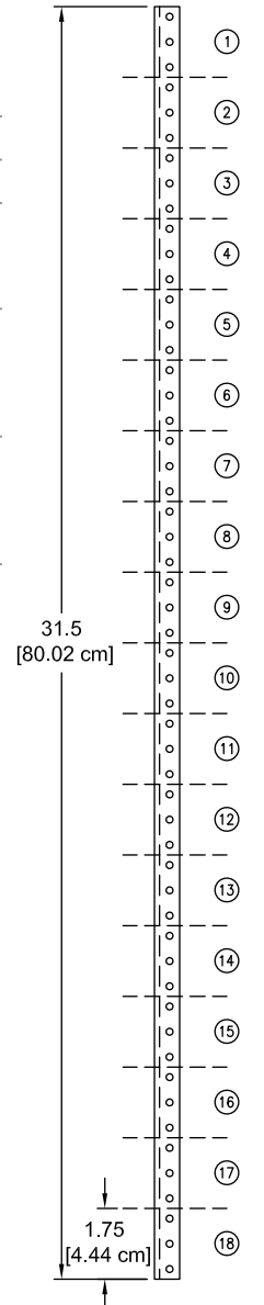
36RU available (18RU front and 18RU rear)
