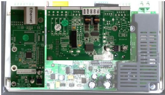
Figure 1-4: Option Board Locations
