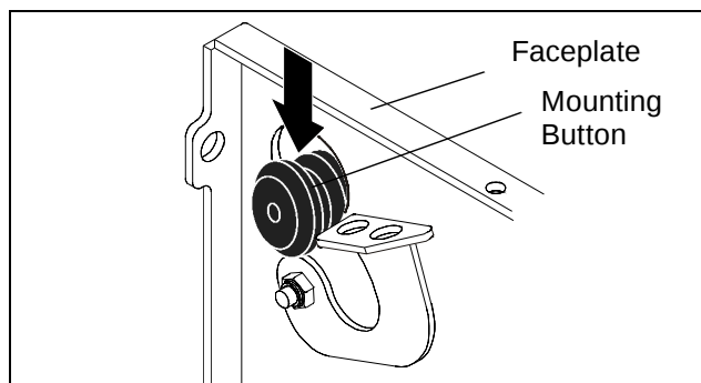
Figure 7: Align Display
