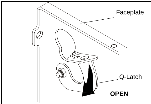
Figure 6: Open Q-Latch
