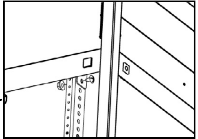
MIDDLE SHELF ATTACHMENT
