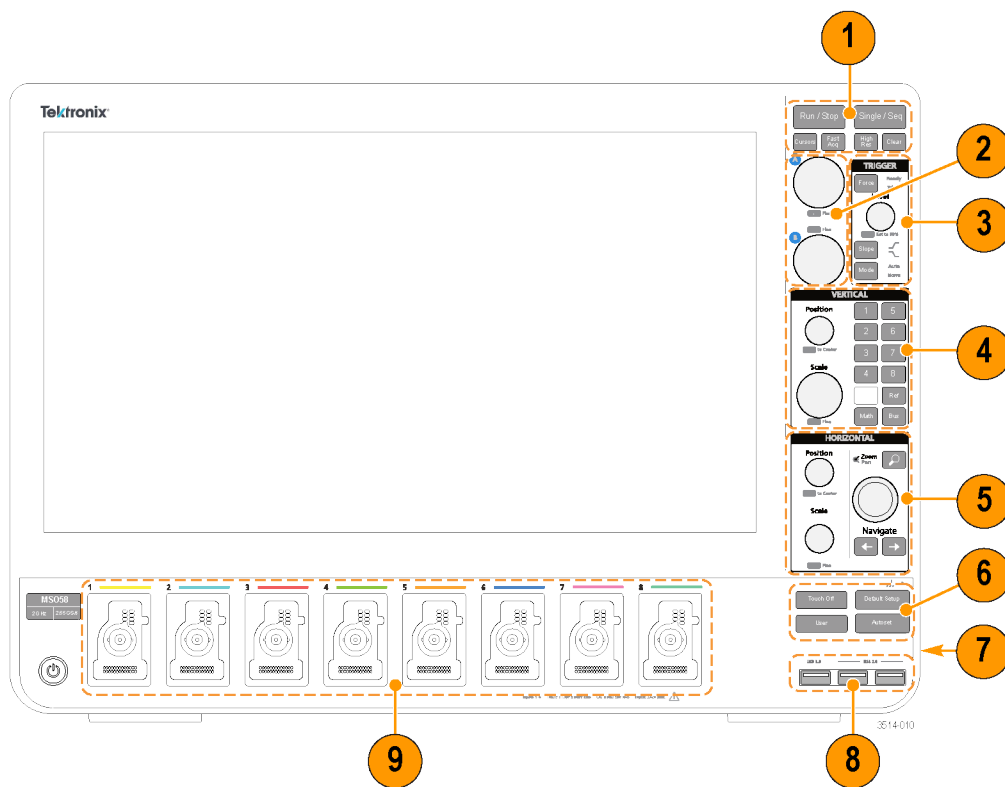
Figure 3: 5 Series MSO controls
