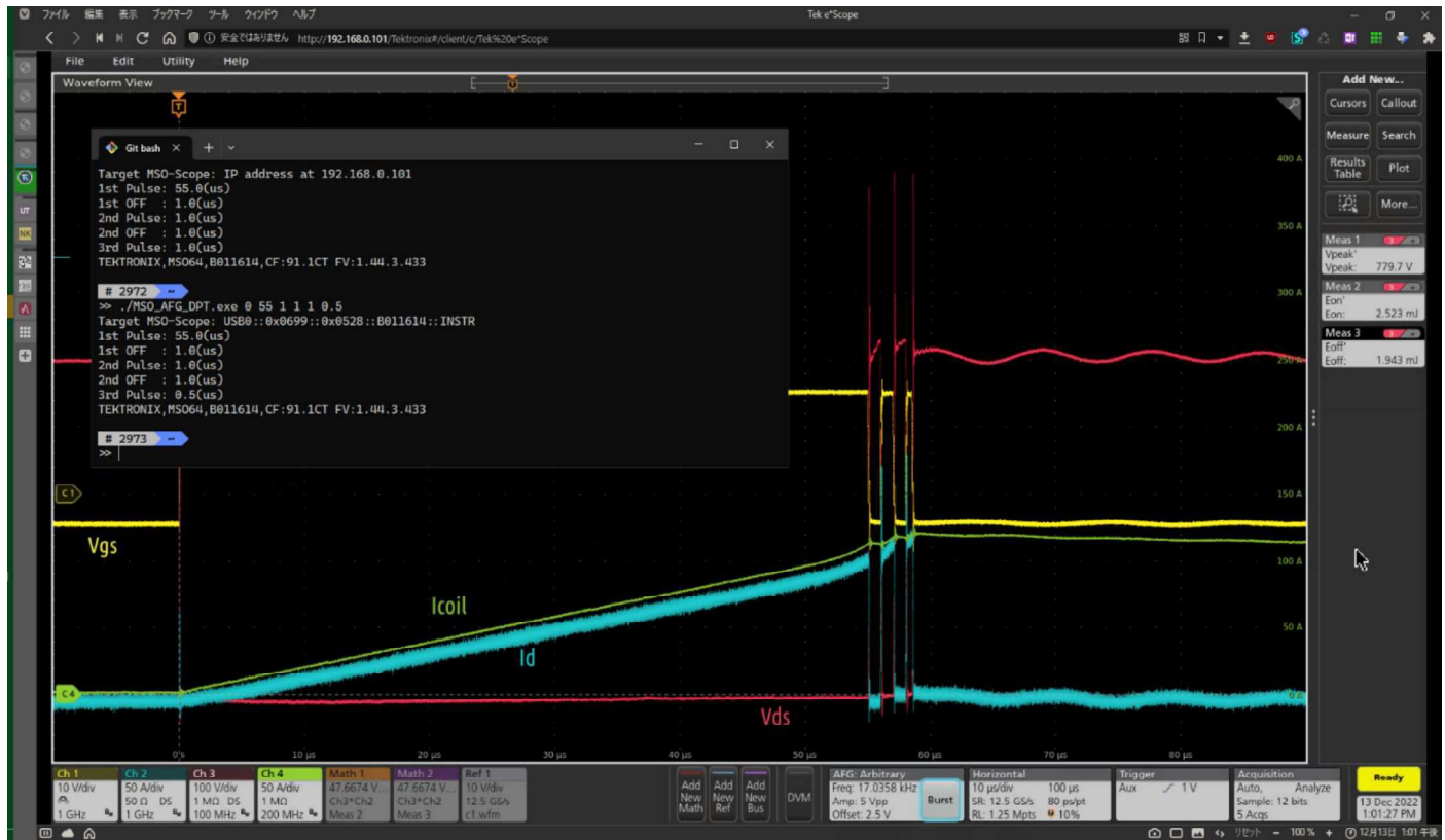
Figure 11: 3-pulse DPT with 100 ns resolution. The third pulse is 0.5 μs wide. When compared to the test in Figure 10, one can see that the third pulse is half as wide.
