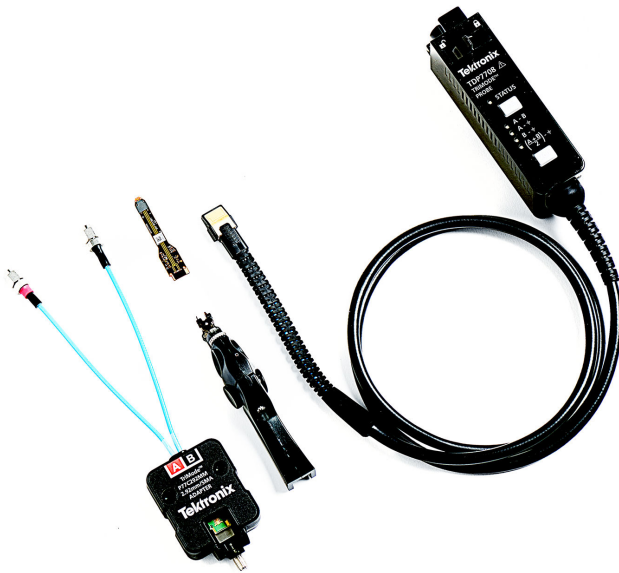
TDP7700 Series probe with a selection of available tips
