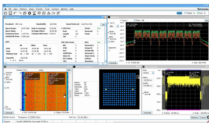
Easy analysis of WLAN 802.11ac transmitter with a WLAN preset that provides spectral emission mask, constellation diagram, and decoded burst information.
