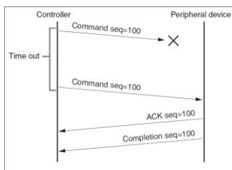
Sequence chart when command lost
