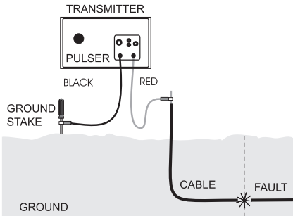
Figure 1. Transmitter Setup
