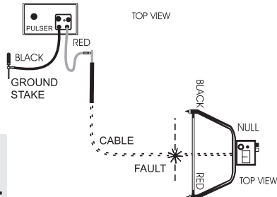
Figure 5. Nulling Receiver - Second Time
