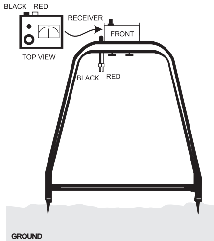
Figure 2. Receiver Setup
