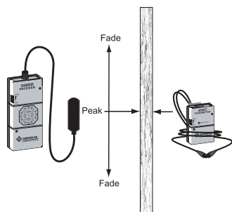
Fig. 07 - Pinpointing Drill Sites
