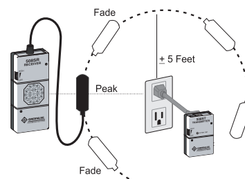
Fig. 03 - Tracking Behind Walls
