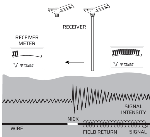
Figure 4. Locating Wire Nick
