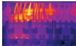
Maintaining plants: Identify excessively high temperatures in circuit breakers and electrical components before breakdowns can occur.
