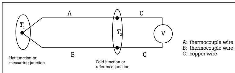
Figure 1: Thermocouple construction.
