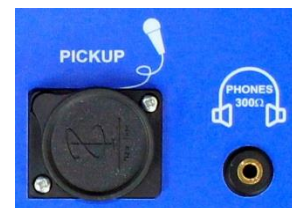
Figure 7 Pickup & Headphones Connection
