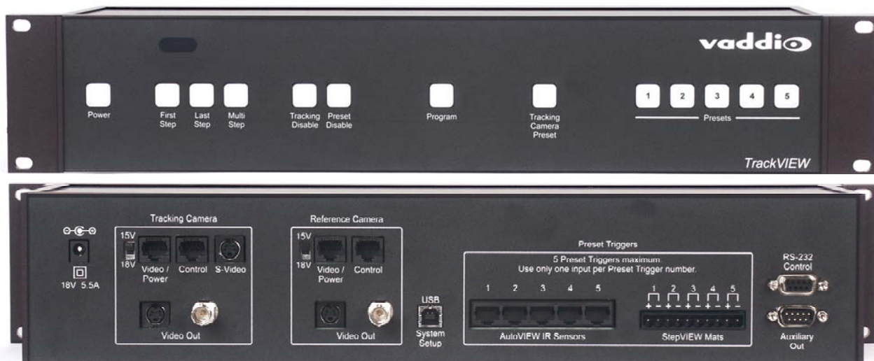
Figure 1: Front and Back Panels of Vaddio TrackVIEW System Controller
