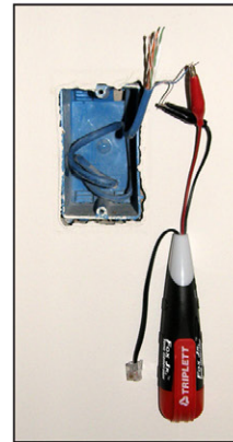
Alligator clips for easy toning of any 2 pair
