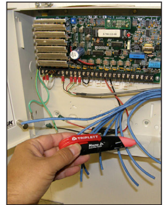
Signal strength LED to help determine proper cable location in a bundle
