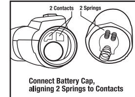
Push IN and Rotate Cap back onto Tester Body
