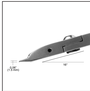
Standard Profile
