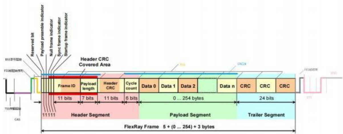
Figure 4-1: FlexRay frame format.
