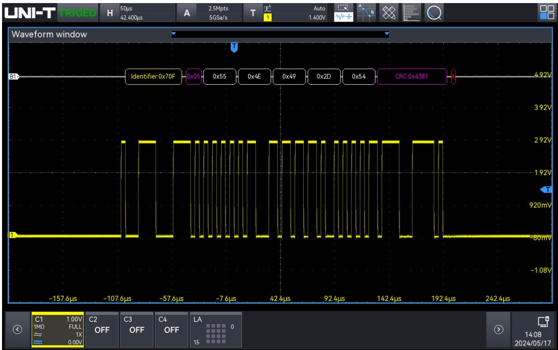
CAN trigger and decoding result
