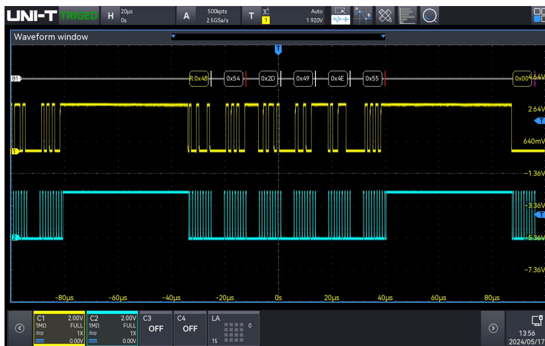
I 2 C trigger and decoding
