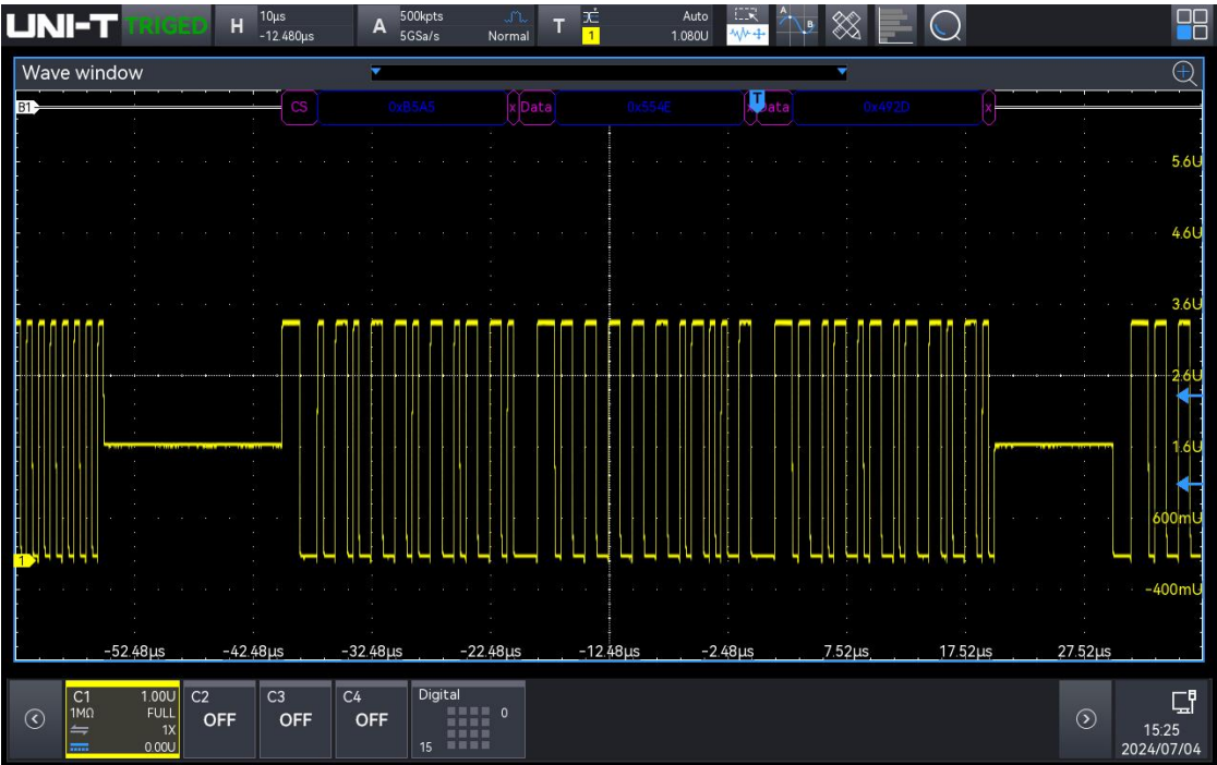
1553B data block trigger and decoding
