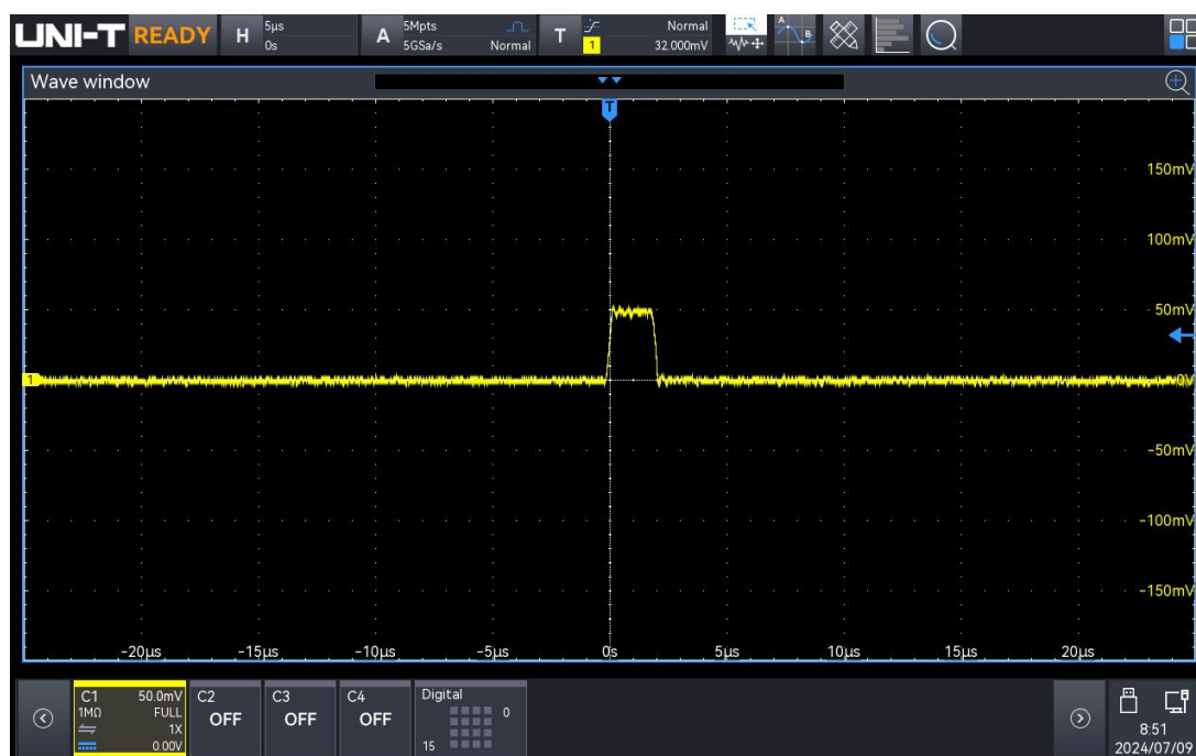
Single-shot pulse with ringing
