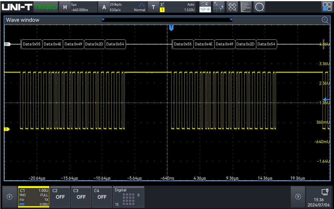
Manchester trigger and decoding
