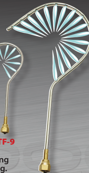
CAP'N HOOK ® MTF-17 17 Flame Tip Capable of Brazing 3" Copper Tubing.
