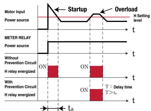
Relay Energizing Timing Chart
