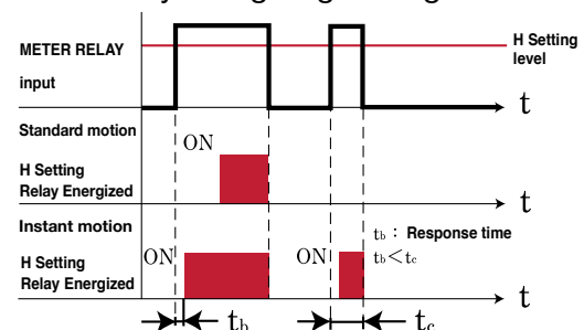
Relay Energizing Timing Chart
