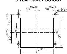
2104 Panel Cutout
