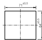
2103 Panel Cutout
