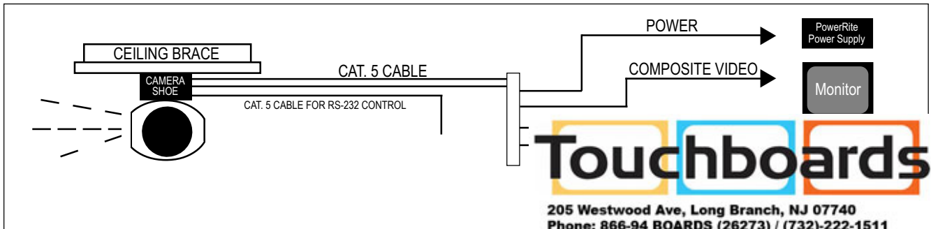
Figure 2 – EZCamera cable system with a Quick-connect and RS-232
