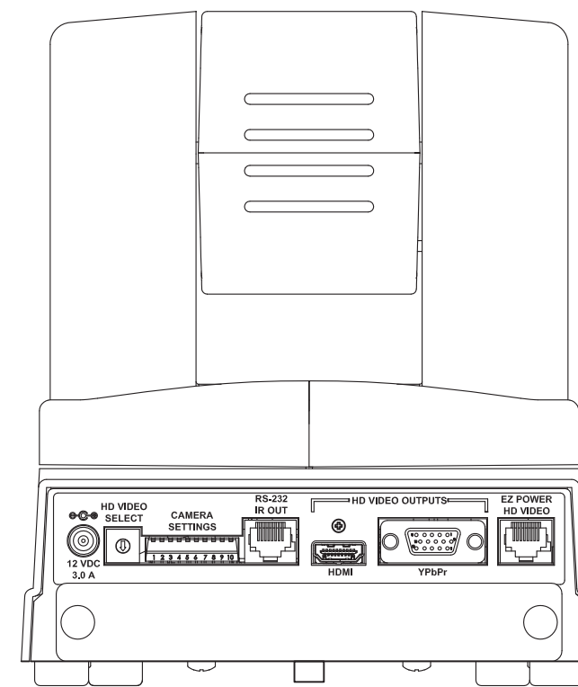
REAR VIEW NO SLOT CARD - COVER ONLY
