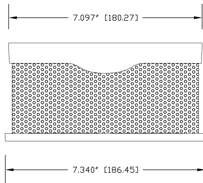
SIDE VIEW 1
