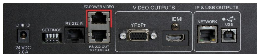
Images: Quick-Connect USB Front Panel (up) and Rear Panel (below)
