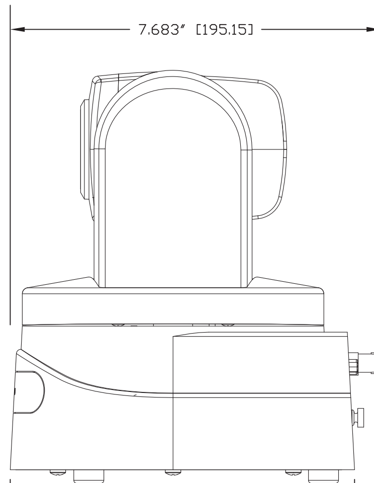
SIDE VIEW
