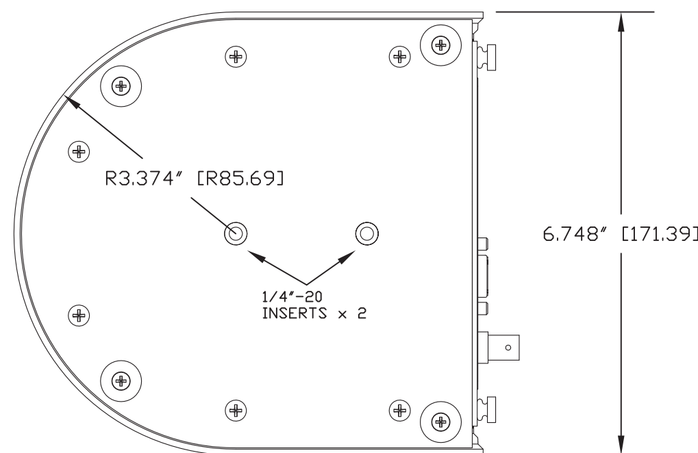
BOTTOM VIEW
