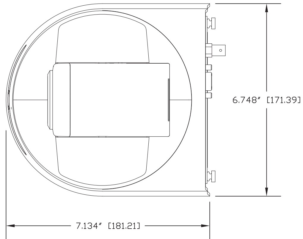
TOP VIEW
