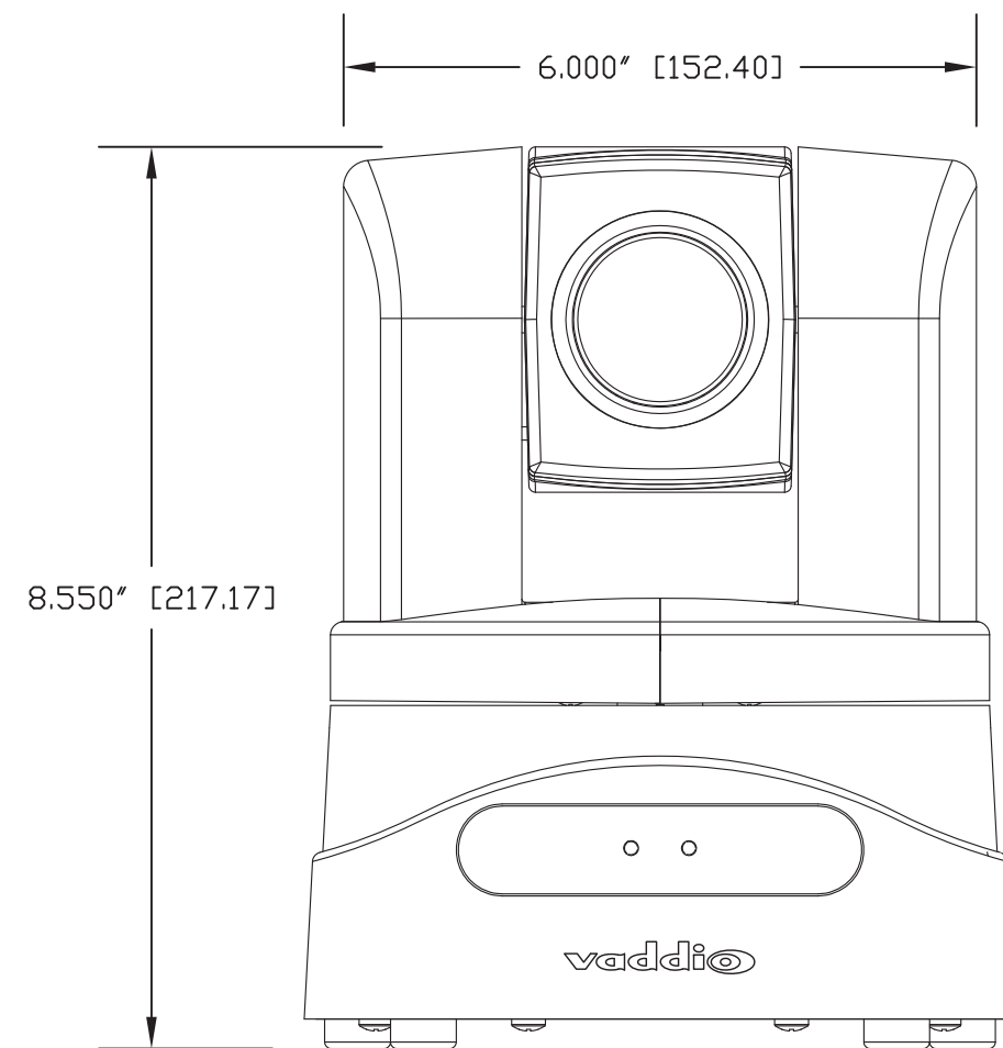
FRONT VIEW
