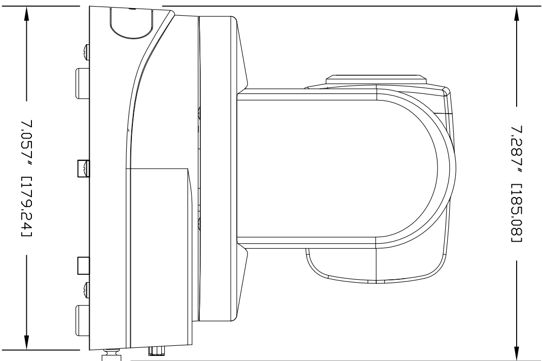
SIDE VIEW
