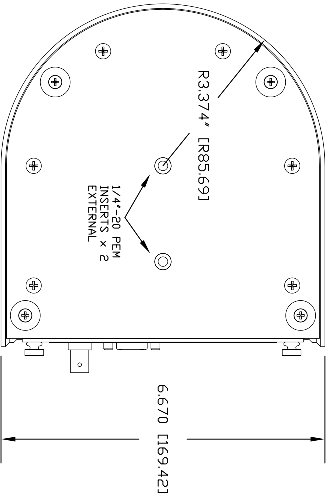
BOTTOM VIEW
